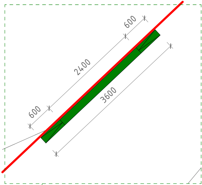
02/EXISTING CALLOUT 1: 50
