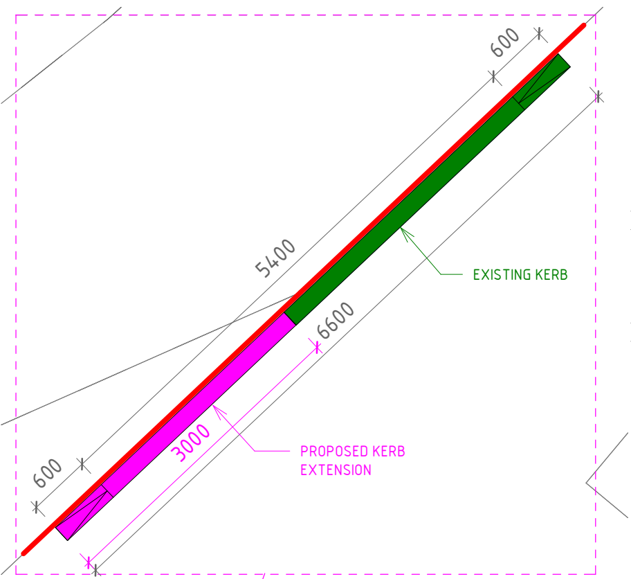
02/PROPOSED CALLOUT 1: 50
