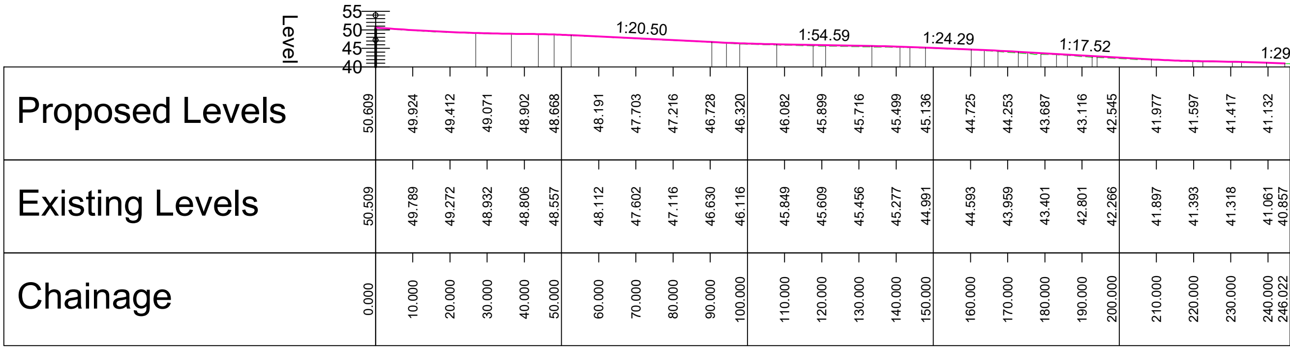
PHASE 3 CYCLEWAY ALIGNMENT - LONGSECTION SCALE: H 1:1000,V 1:1000. DATUM: 40.000
