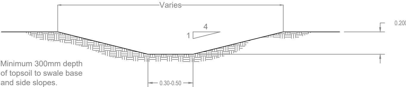
Typical Swale Detail
