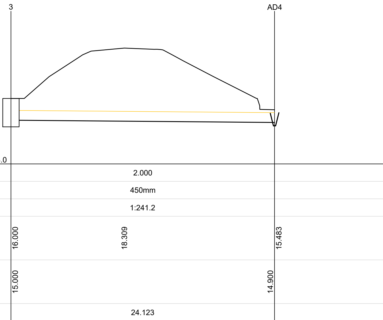
Section through Acoustic Bund.
