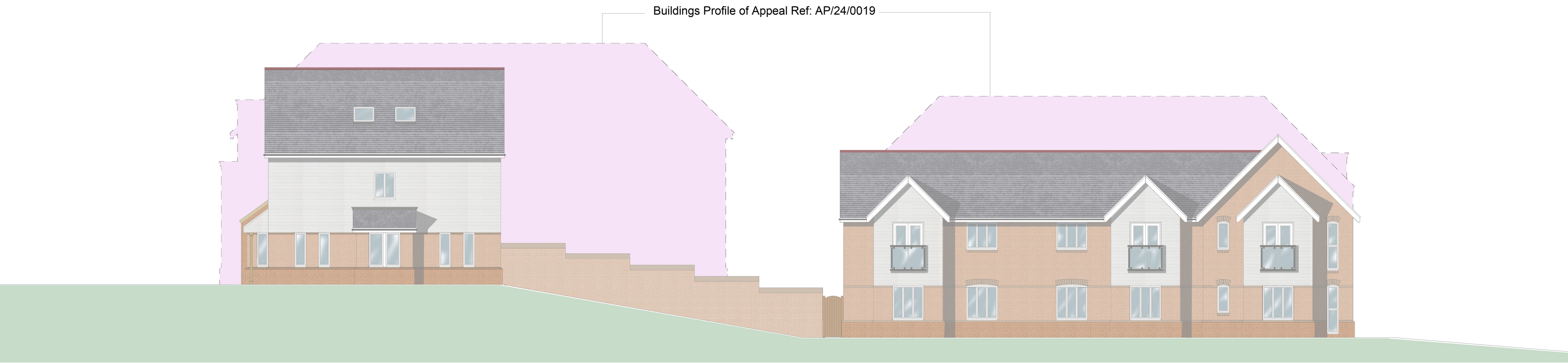
South Elevation (Bowden Way) (In Context with Buildings Profile of Appeal Ref: AP/24/0019)
