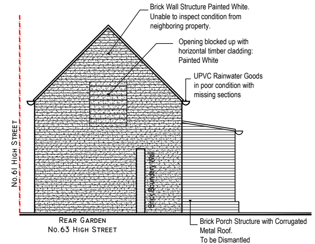
EXISTING EAST SIDE ELEVATION
