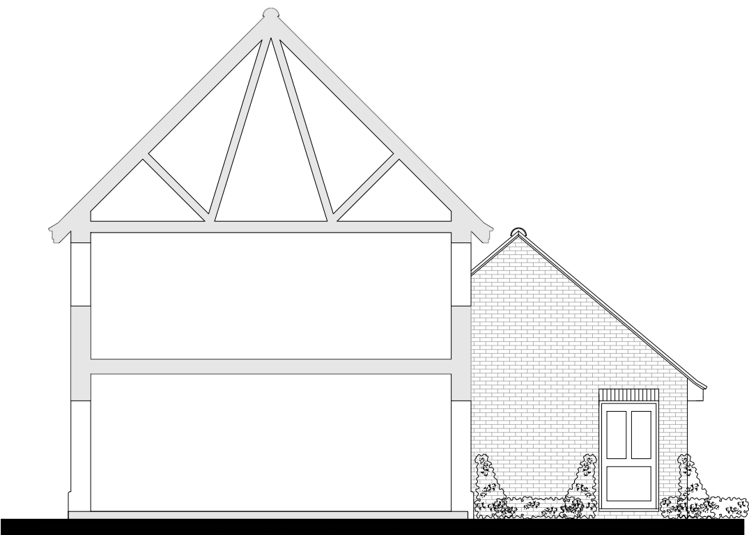
SECTION / SIDE ELEVATION
