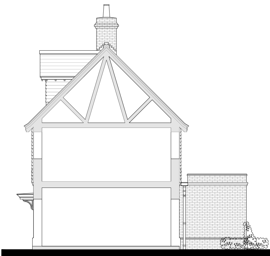
SECTION / SIDE ELEVATION
