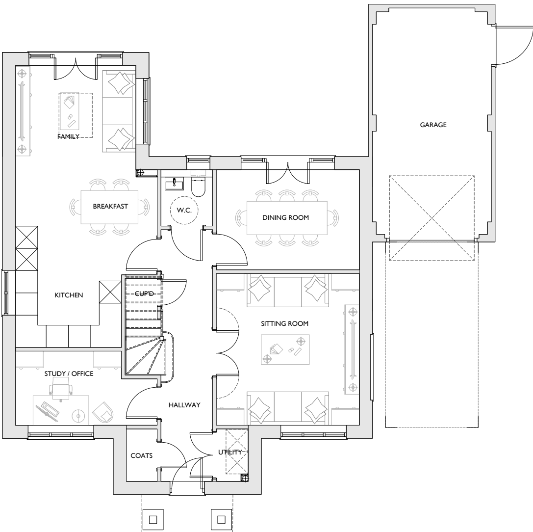
GROUND FLOOR PLAN 2,015 sqft PLOT 7
