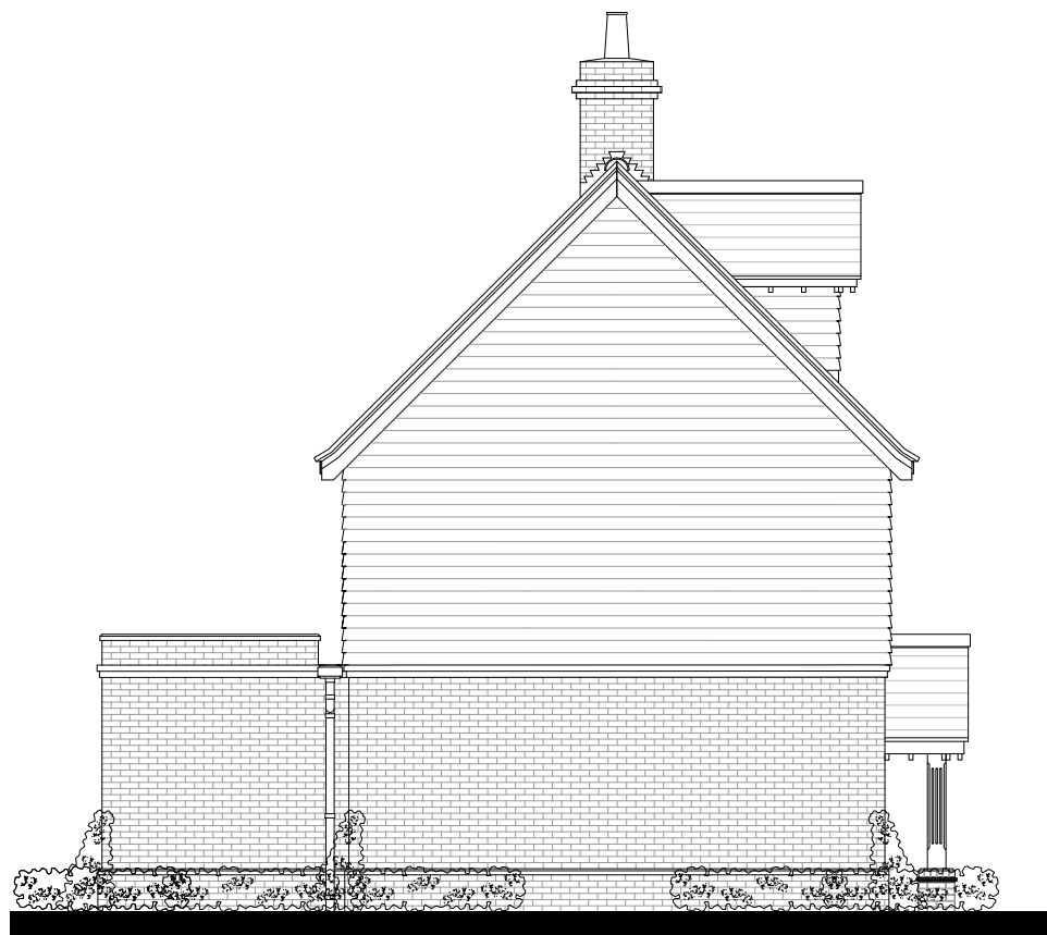
SIDE ELEVATION
