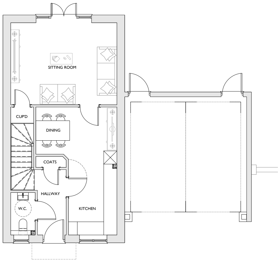
GROUND FLOOR PLAN 1,001 sqft PLOT 13
