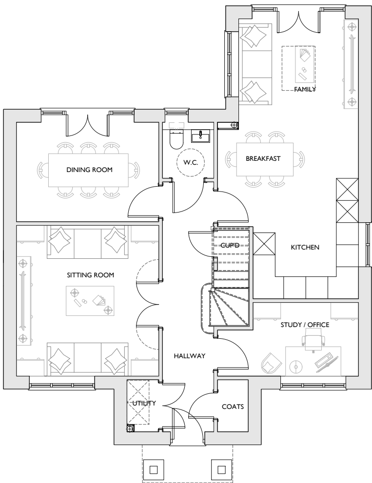
GROUND FLOOR PLAN 2,015 sqft PLOT 15
