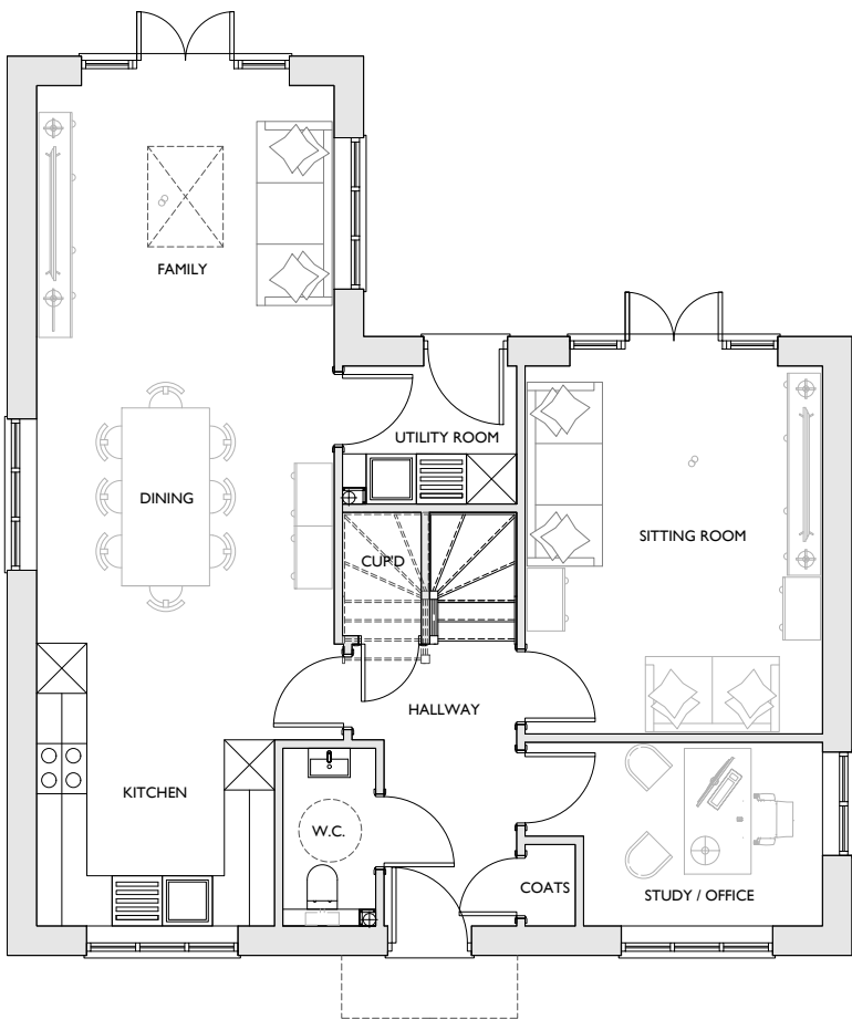
GROUND FLOOR PLAN 1,896 SQFT PLOT 16
