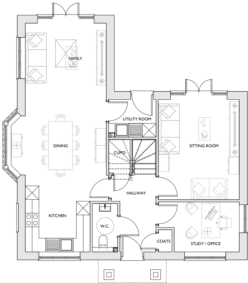
GROUND FLOOR PLAN 1,498 SQFT PLOT 19 (24 HANDED)
