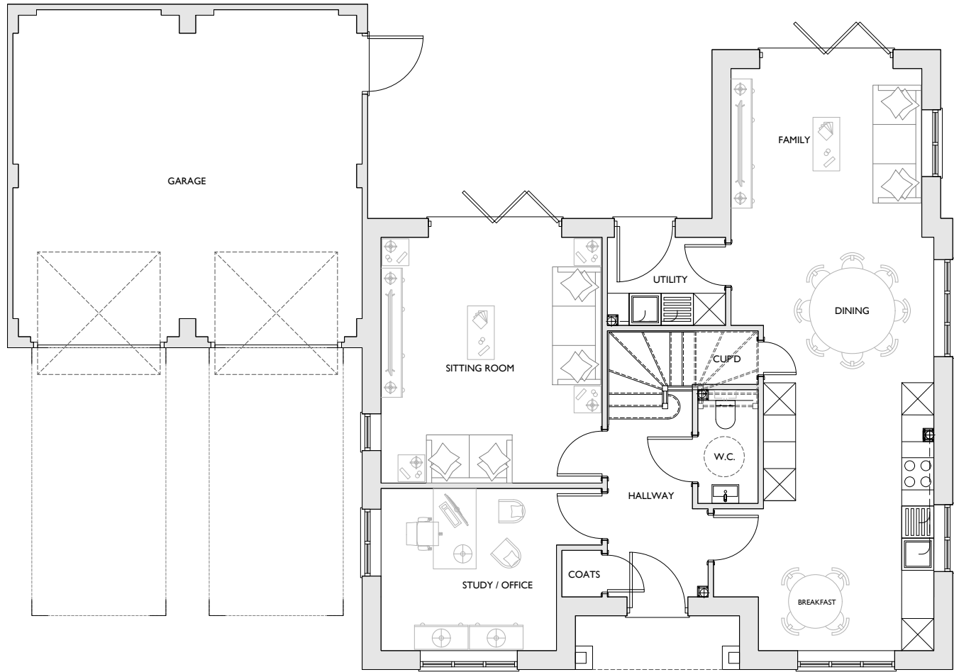
GROUND FLOOR PLAN 2295 sqft PLOTS 20 & 23(HANDED)
