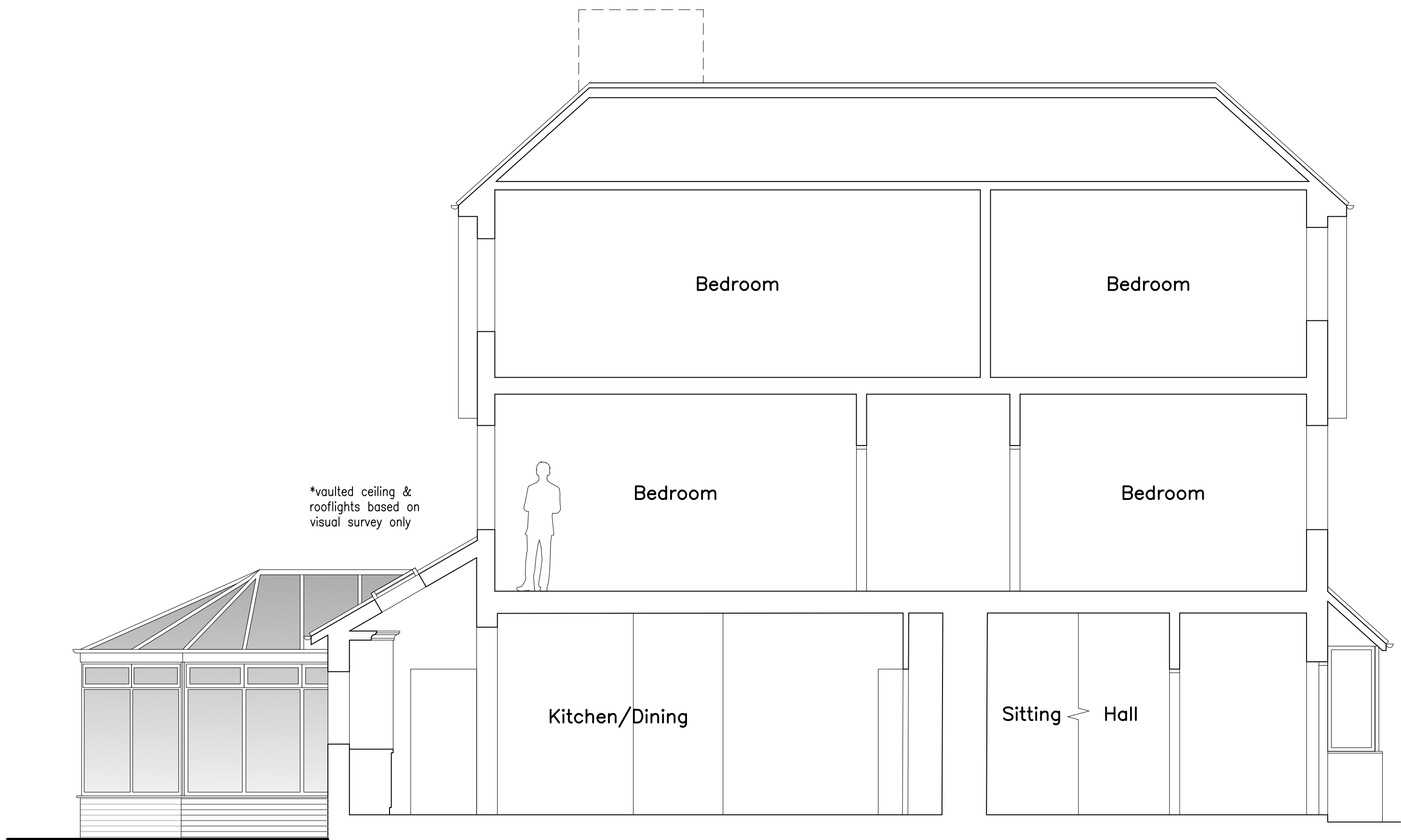
Section B-B 1:50
