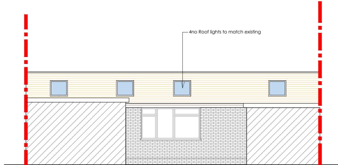
PROPOSED SECTIONAL ELEVATION A Scale 1:100
