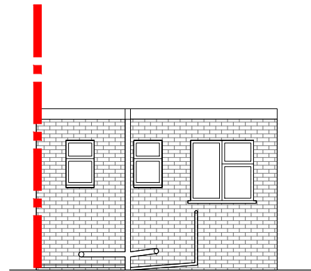
PROPOSED SECTIONAL ELEVATION B Scale 1:100
