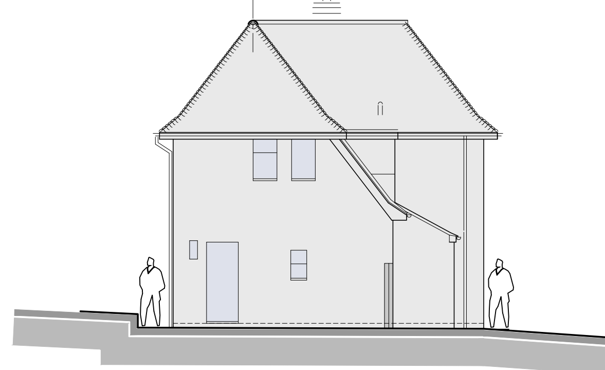
Existing Side (South) Elevation
