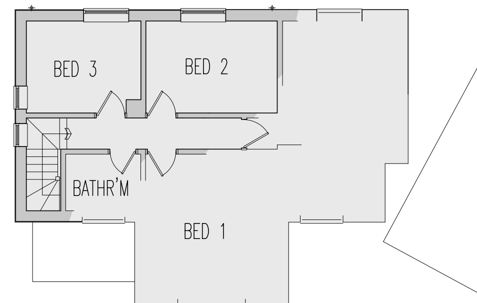
Existing First Floor Plan FOR REFERENCE
