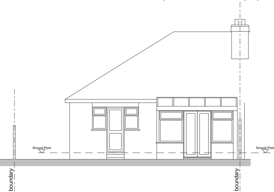
NORTH ELEVATION 1:100
