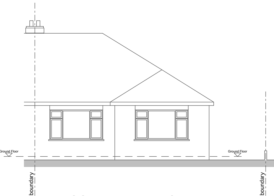
SOUTH ELEVATION 1:100
