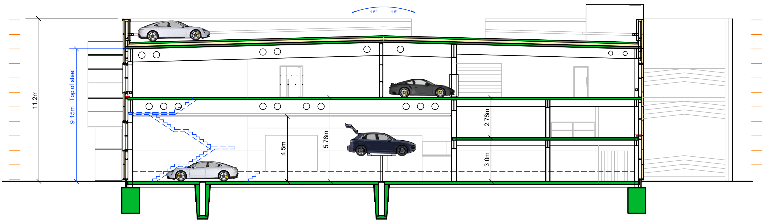
BUILDING CROSS SECTION
