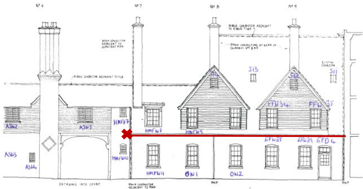
GUEST WING AT MAIN COURTYARD (WEST ELEVATION)
