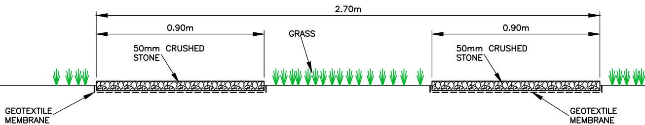
- TYPICAL SECTION THROUGH PROPOSED ACCESS TRACK - 1:20 -
