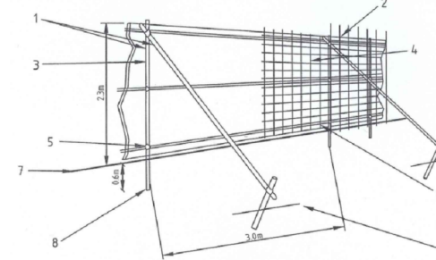
BS:5837 Figure 2 - Tree Protection Fencing structure around RPA
