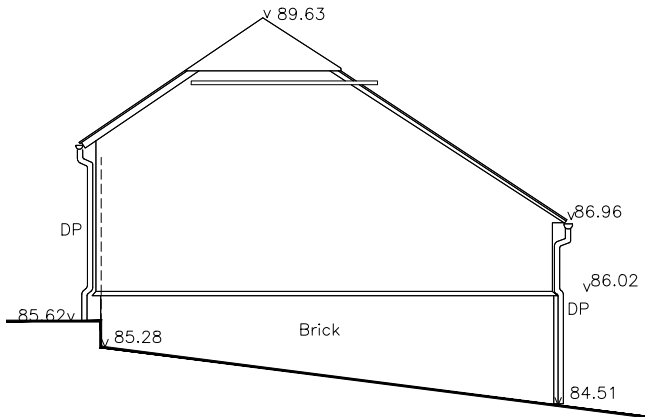
West elevation EXISTING + PROPOSED
