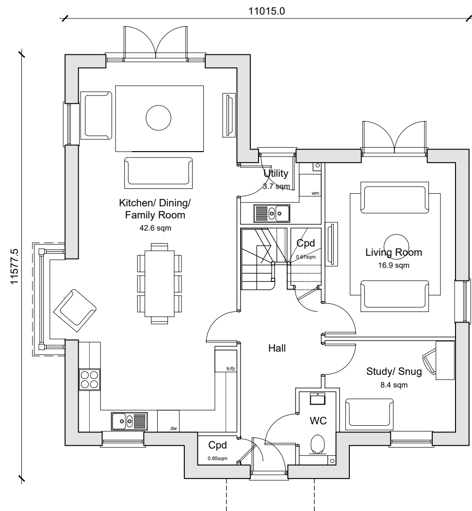
Ground Floor Plan H154 4-Bedroom 8-Person House 169.46sqm / 1824sqft GFA, in house A minimum of four storage spaces is provided in accordance with NCRS requirements.
