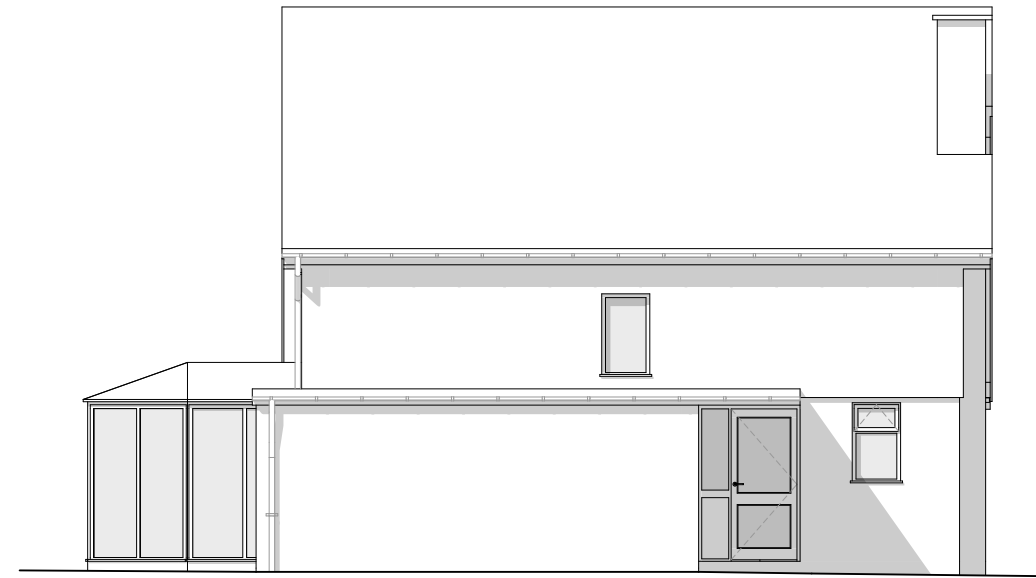
Existing Side (South) Elevation Scale 1:100 @ A3
