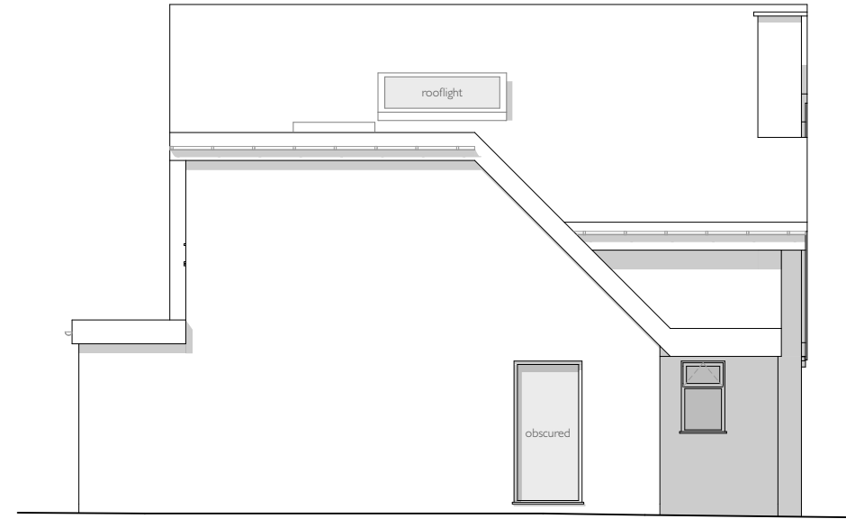
Proposed Side (South) Elevation Scale 1:100 @ A3
