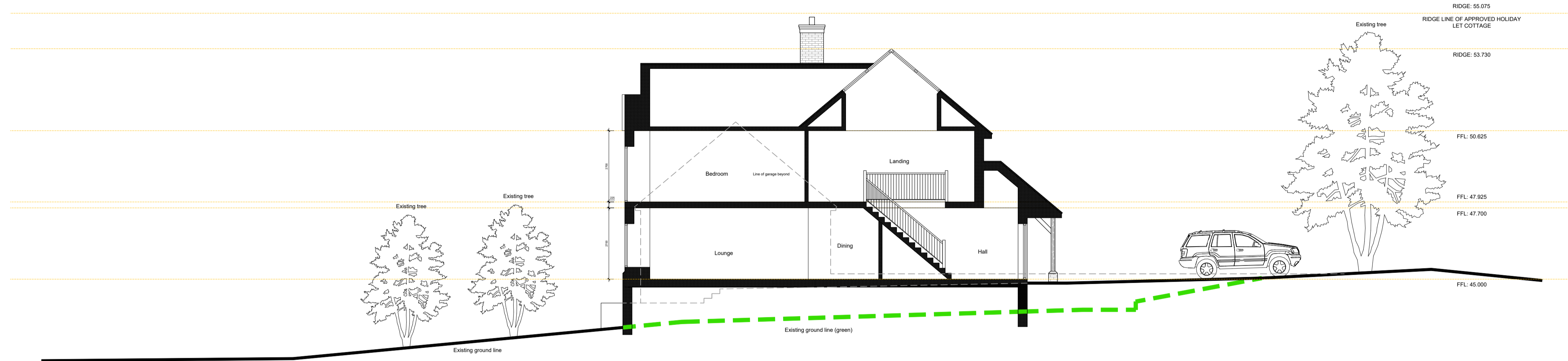
Proposed Site Section 1:100 @ A1
