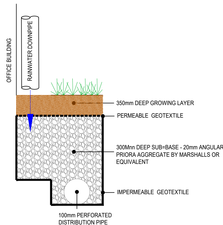
RAINGARDEN DETAIL
