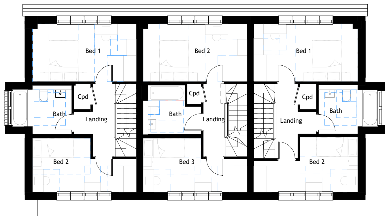
First Floor
