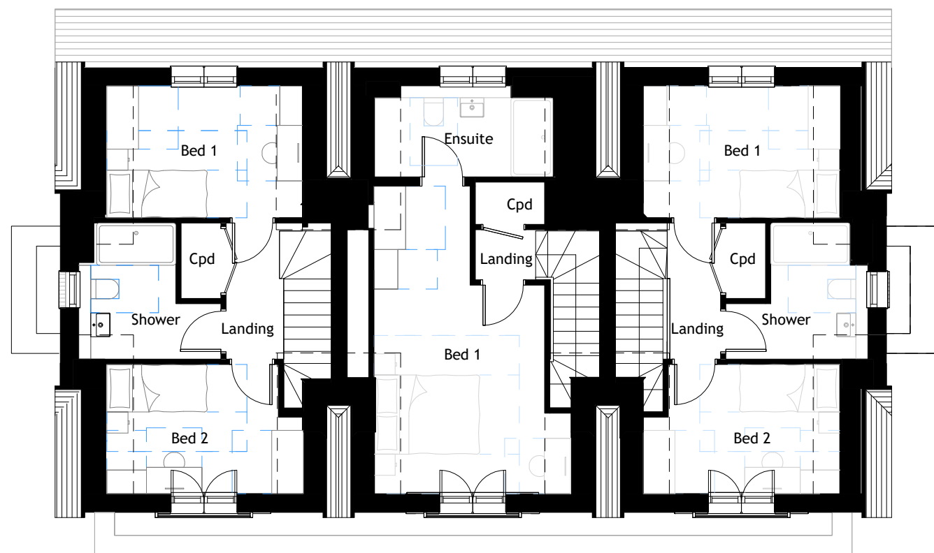
Second Floor
