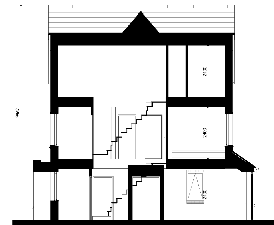
Building Section
