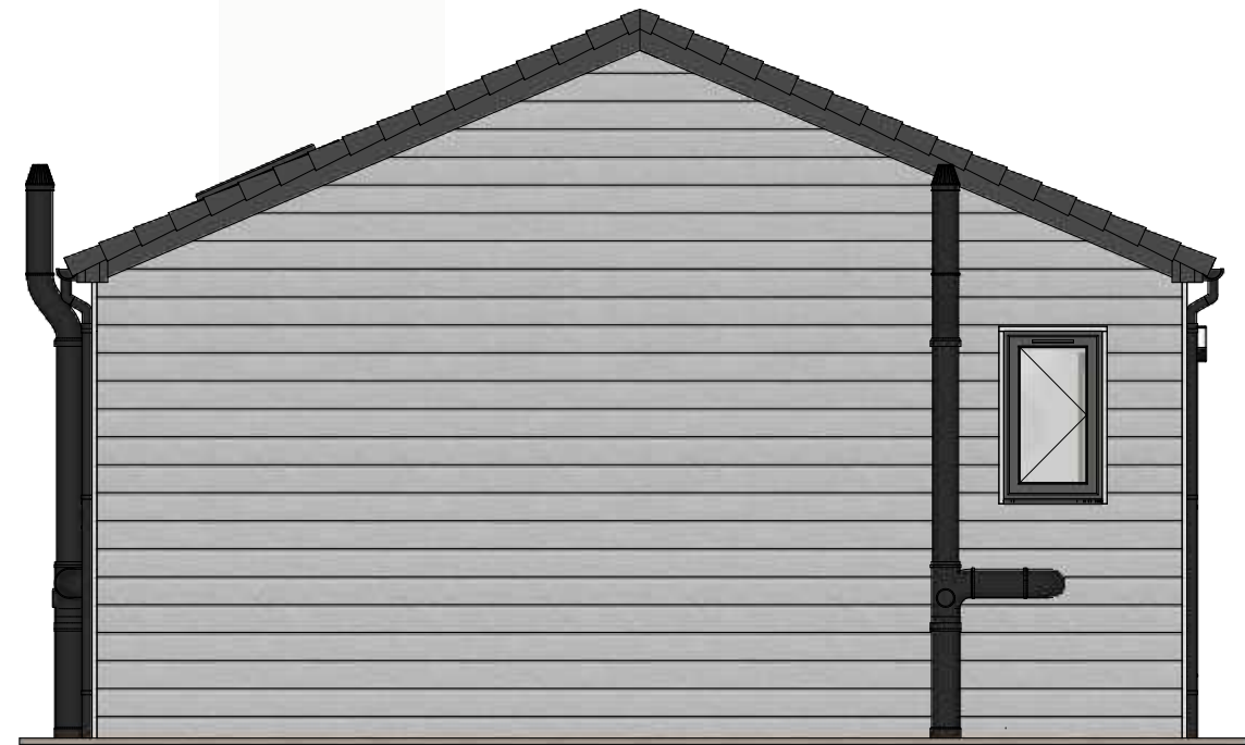
South Elevation
