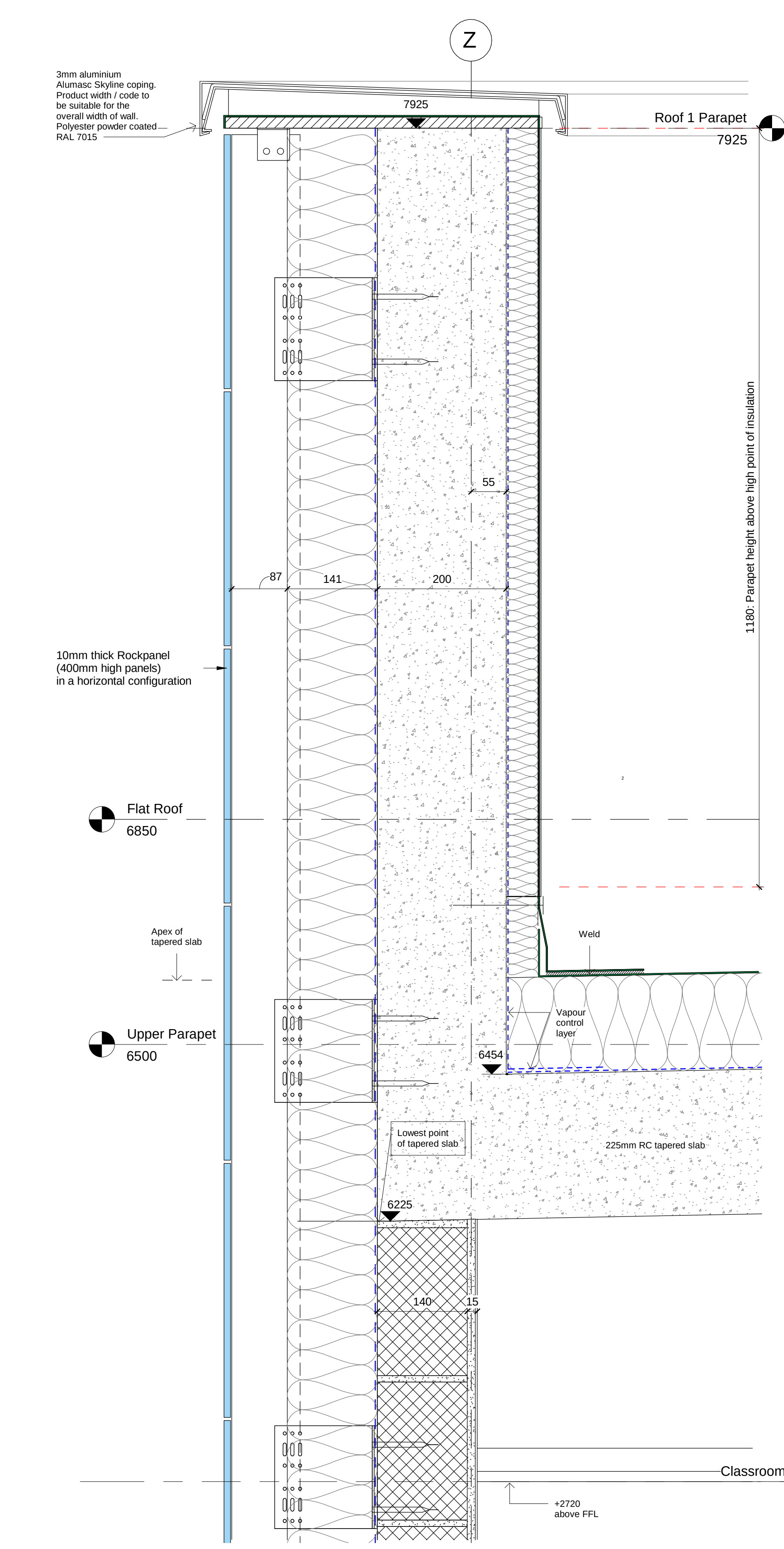
1 Parapet Detail A 1 : 5
