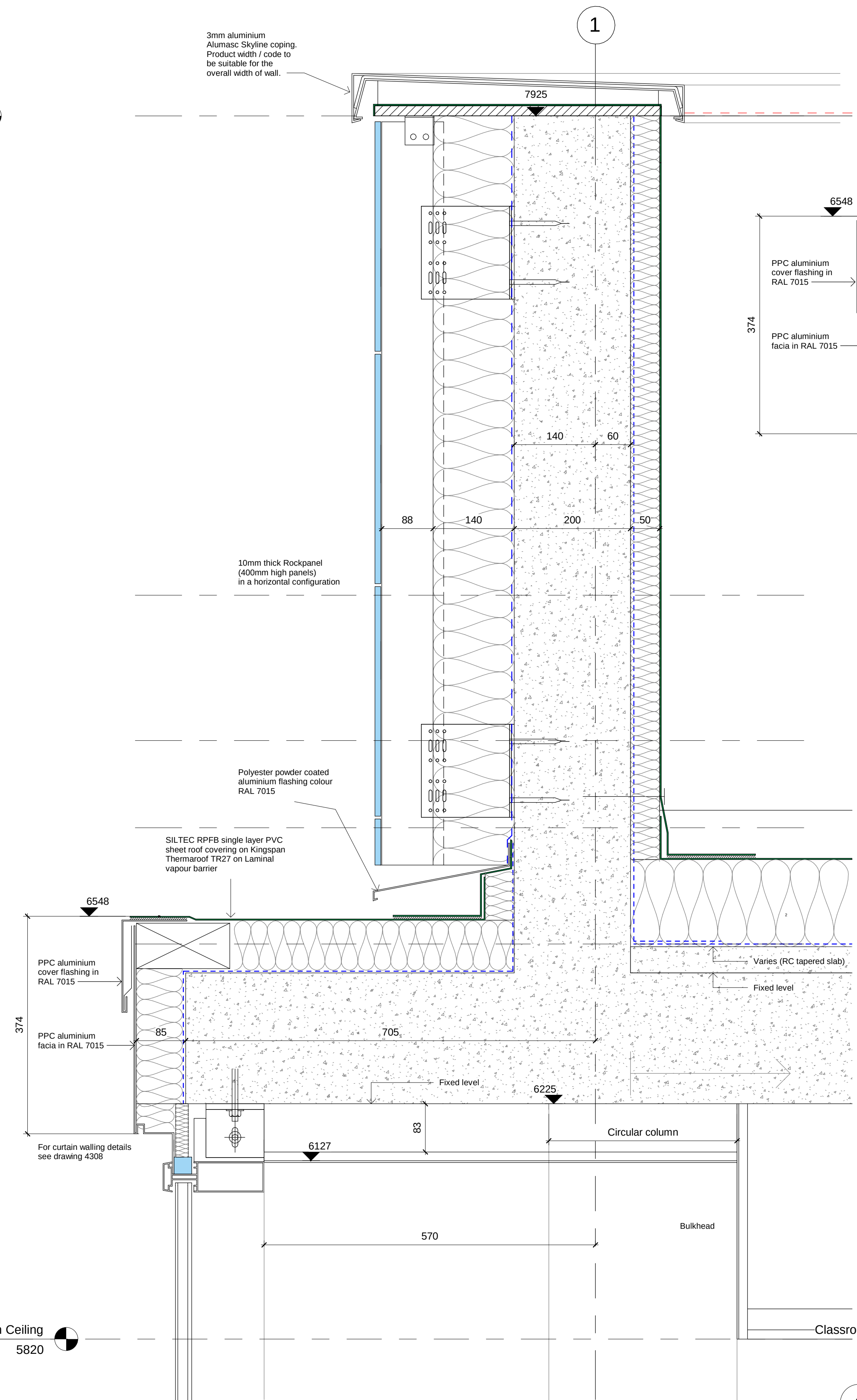
2 Parapet Detail Planning 2 1 : 5
