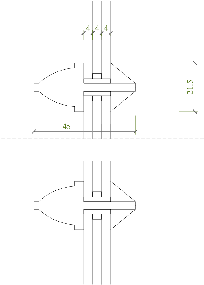
Detail 5a - Painted timber framed windows glazing bar
