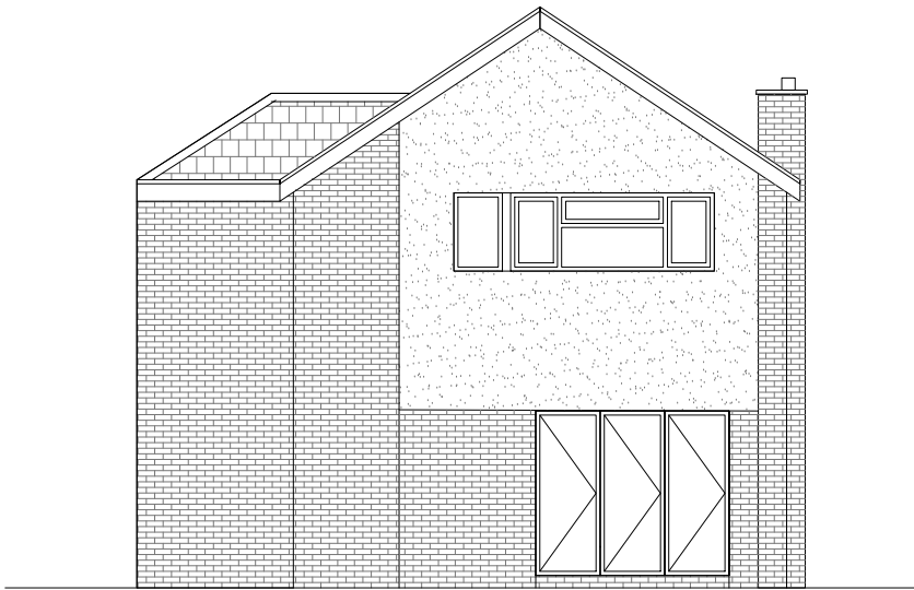
1 EXISTING WEST (REAR) ELEVATION 1:100
