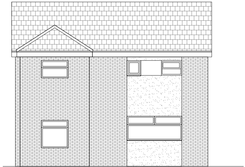
3 EXISTING SOUTH (SIDE) ELEVATION 1:100
