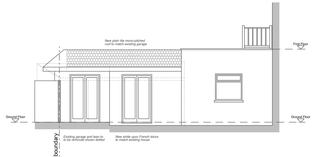
SOUTH ELEVATION 1:100
