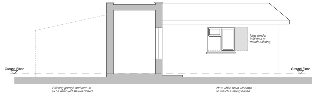
EAST SECTION/ELEVATION 1:100
