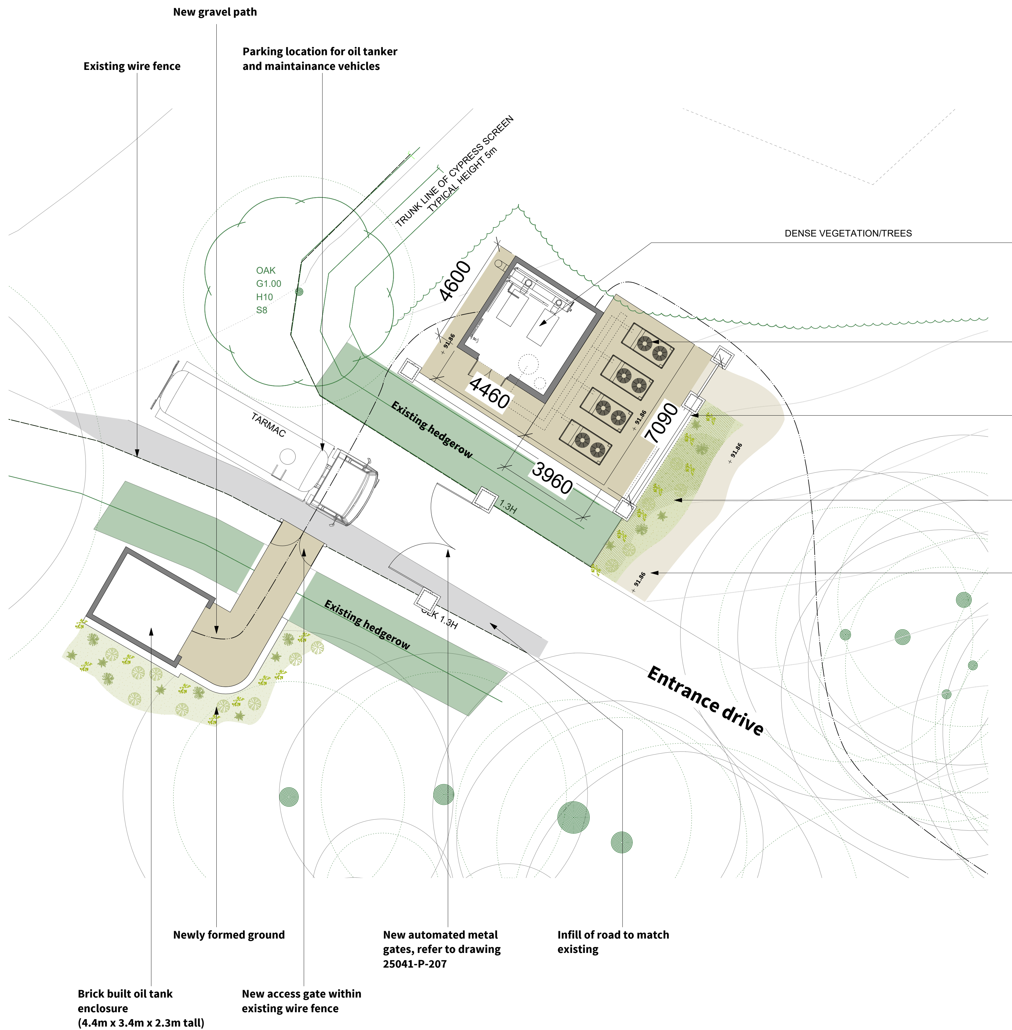
Proposed Garden Plan - Addition of Screened Plant Area 1:100 @A1
