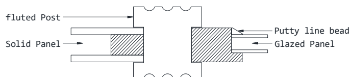
Typical Through Section showing post & panels
