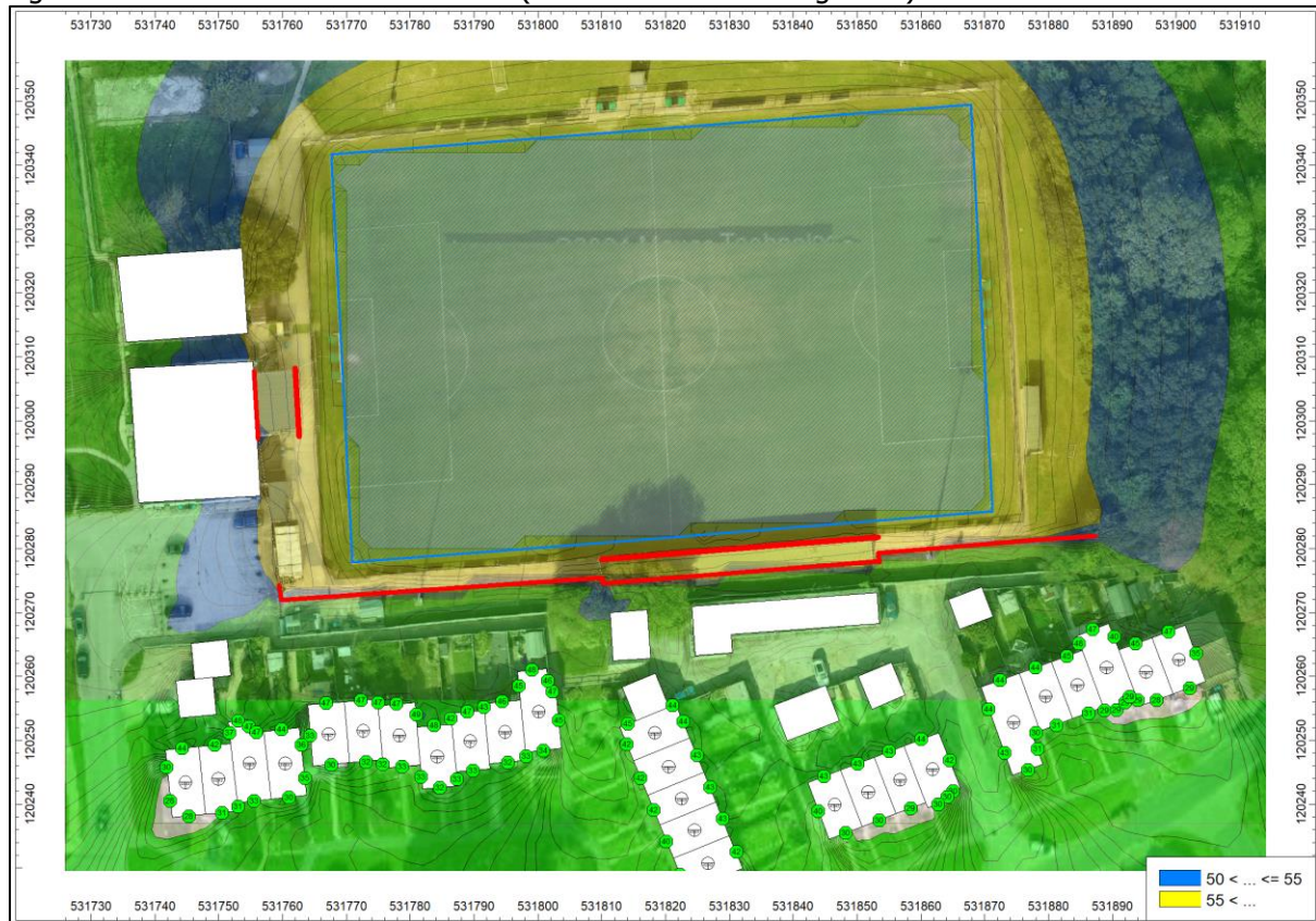
Figure 8: Predicted AGP Noise Emission (1.5 metres above the ground).
