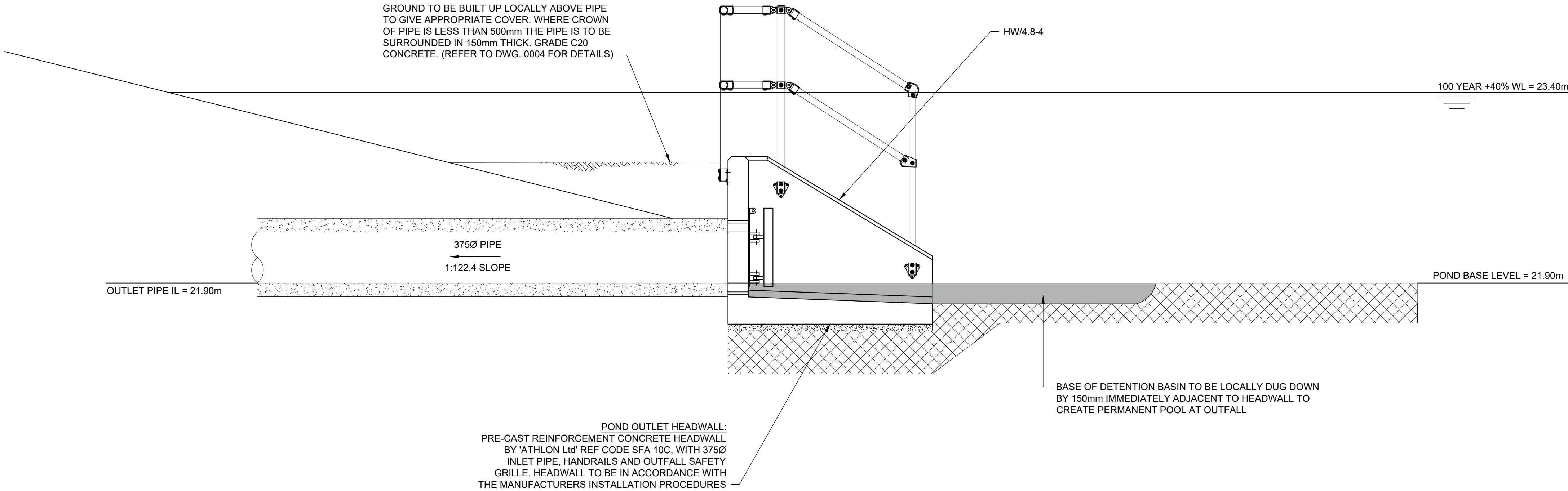
P13 HEADWALL OUTLET LONG SECTION Scale 1:20
