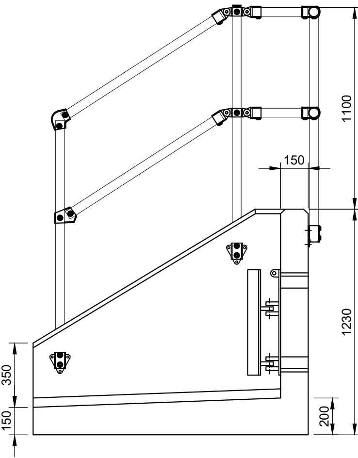
P13 HEADWALL OUTLET DETAILS Scale 1:20
