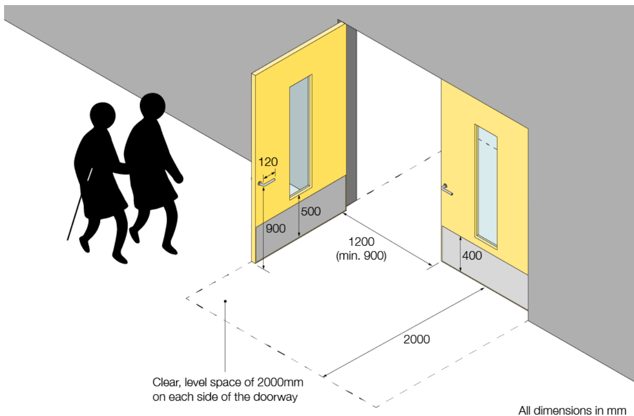
Figure 14: Manually operated doors
