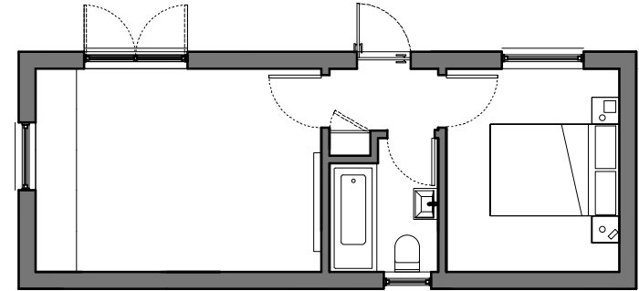
5 PROPOSED 1:100 ANNEXE GENERAL ARRANGEMENT
