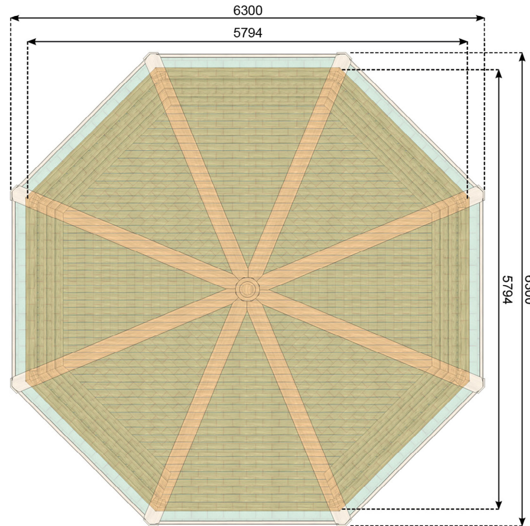
ROOF PLAN
