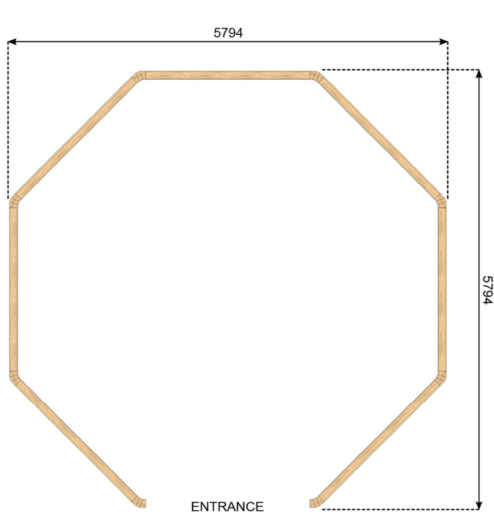
FLOOR PLAN
