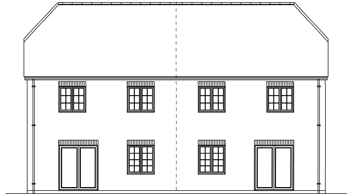
REAR ELEVATION
