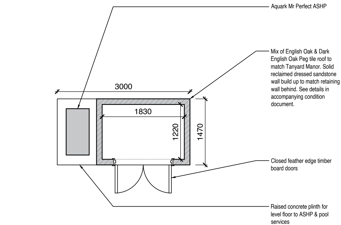
Ground floor plan of pump enclosure & ASHP platform
