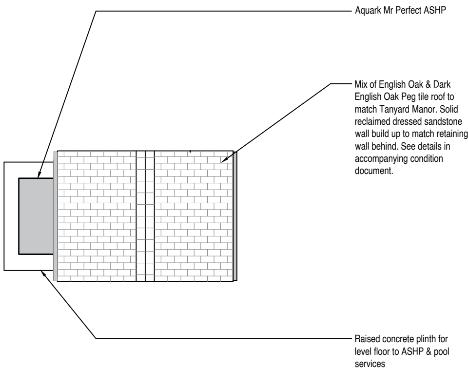
Roof plan of pump enclosure
