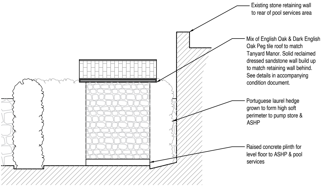
Eastern elevation (Side)
