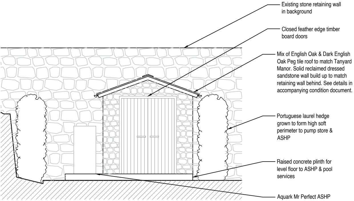
South elevation (Front)
