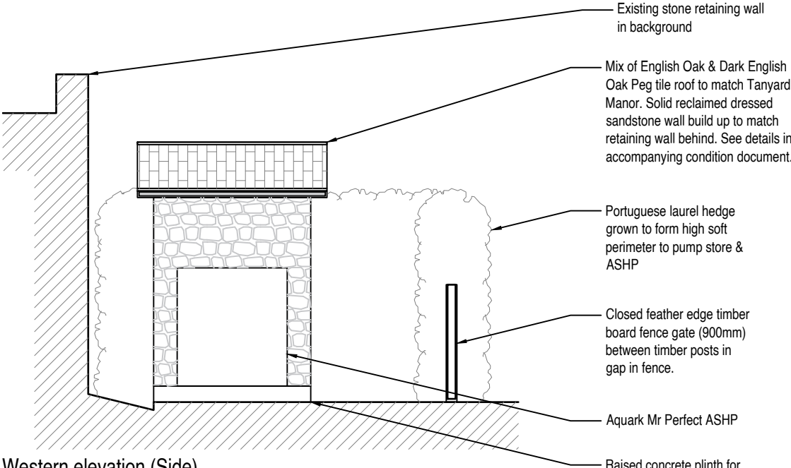
Western elevation (Side)
