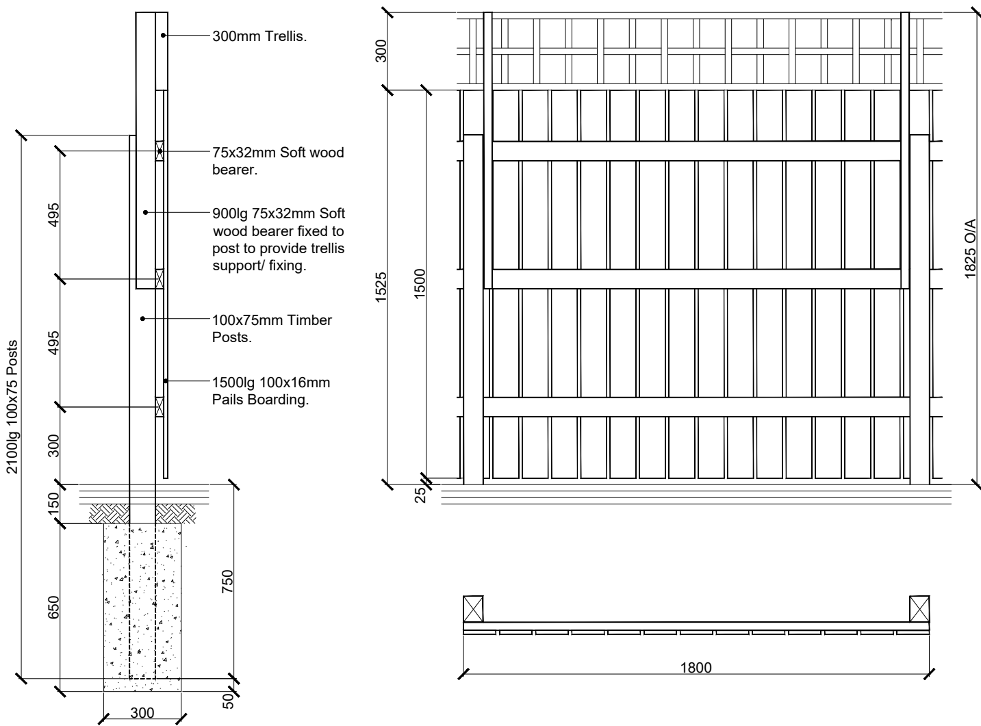
1800MM HIGH BOUNDARY FENCING CLOSE BOARDED - TRELLIS
