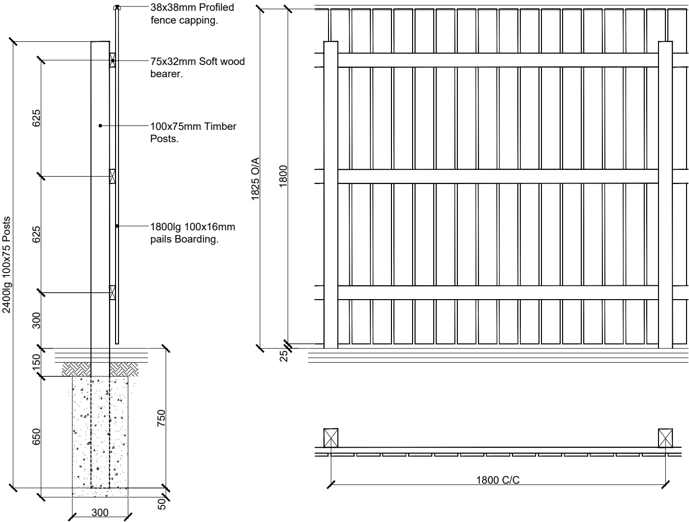
1800MM HIGH BOUNDARY/ PRIVACY FENCING CLOSE BOARDED
