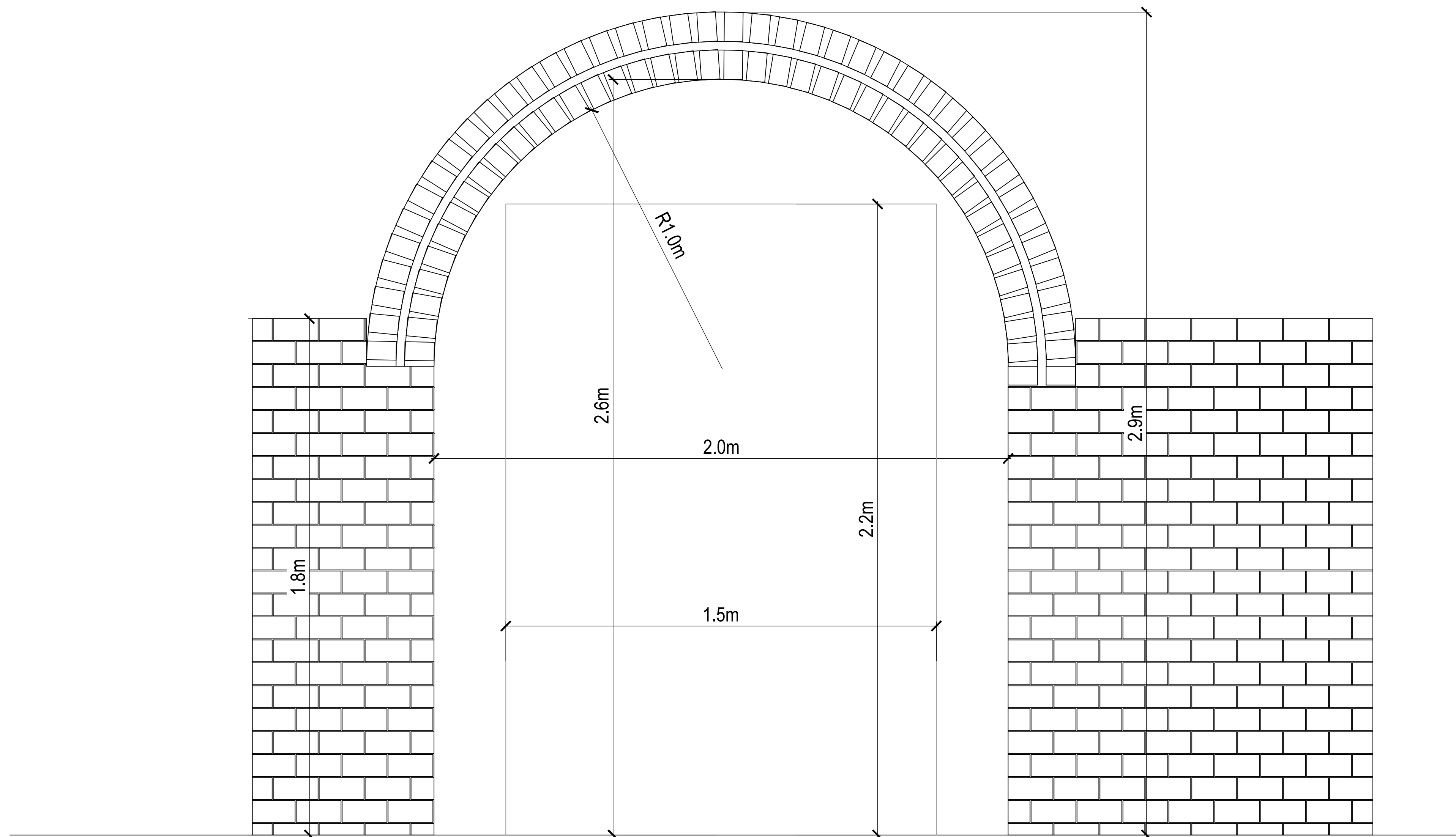
MASONRY BRICK ARCHWAY - 1.8m HIGH WALL (MINIMUM 2.2m HIGH HEAD HEIGHT CLEARANCE)
