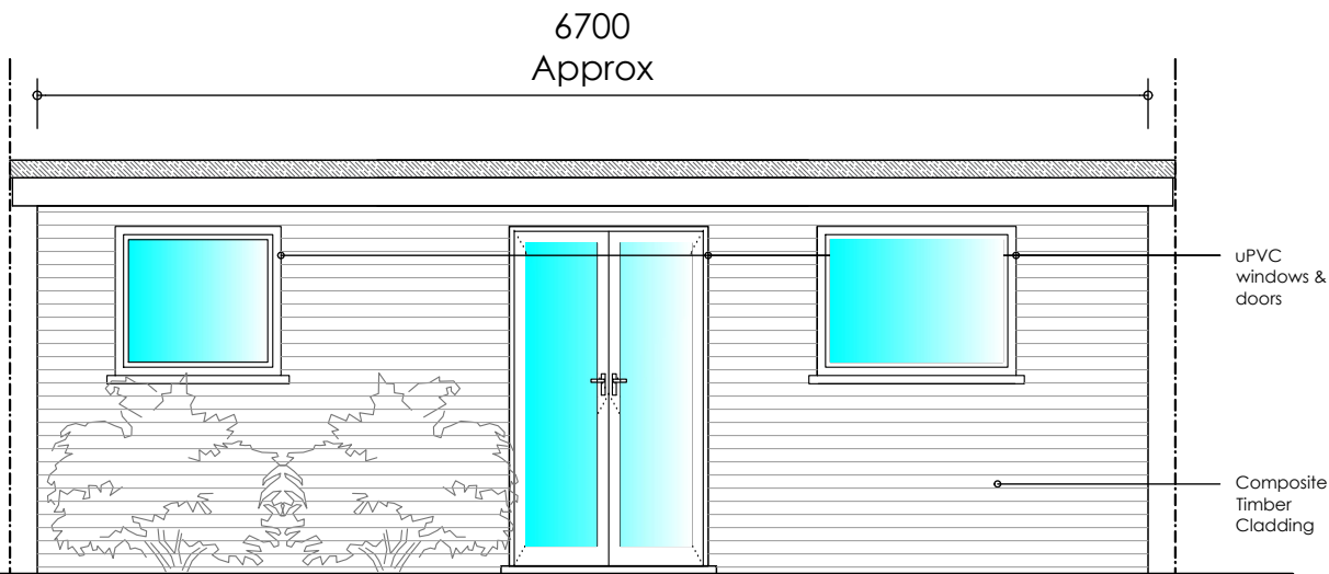
Proposed Front Elevation Scale 1/100@A3
