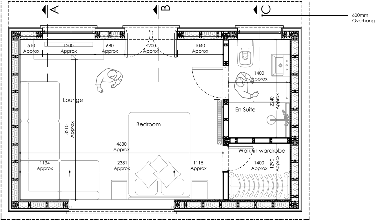
Proposed Garden Room Floor Plan Scale 1/50@A3
