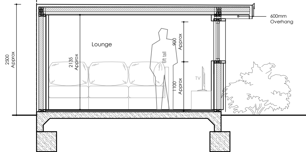
Section B-B Scale 1/50@A3
