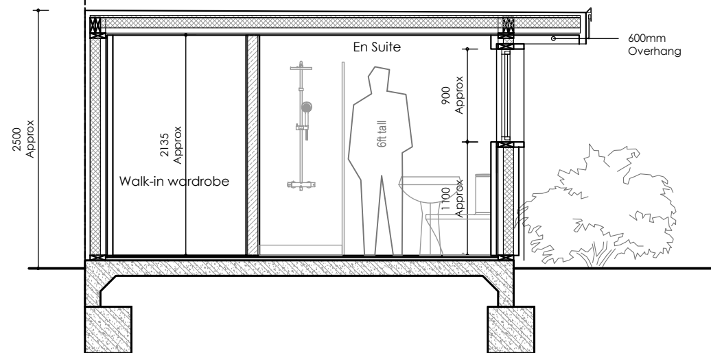
Section C-C Scale 1/50@A3
