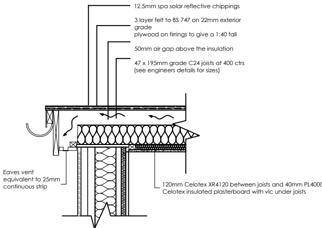
Cold Flat Dormer Roof Ventilation Scale 1/20@A3
