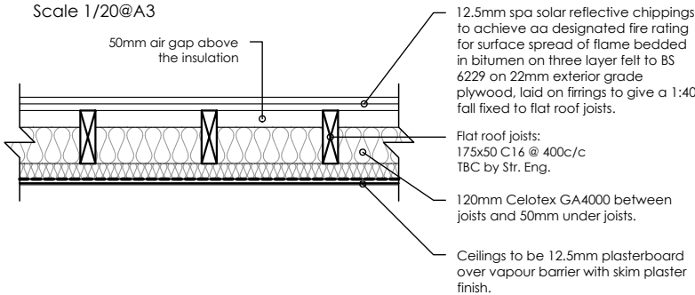
Cold Flat Dormer Roof Scale 1/20@A3
