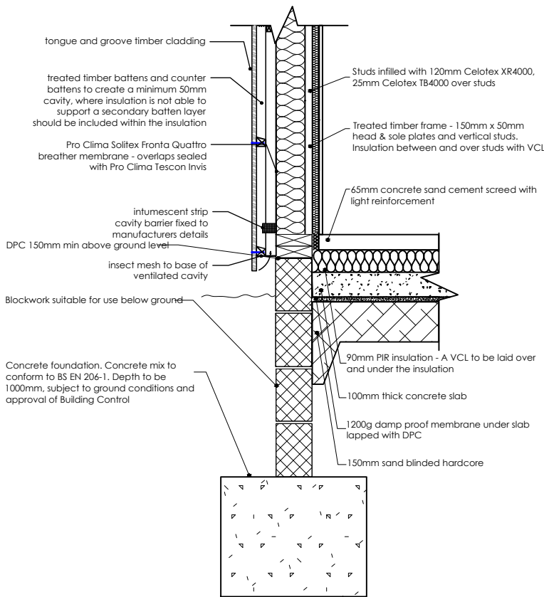
Tile Finish Timber Frame Wall to Solid Floor Scale 1/20@A3
